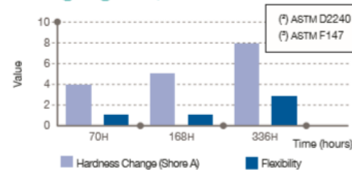
Heat ageing data, air @ 250°C (2,3)
